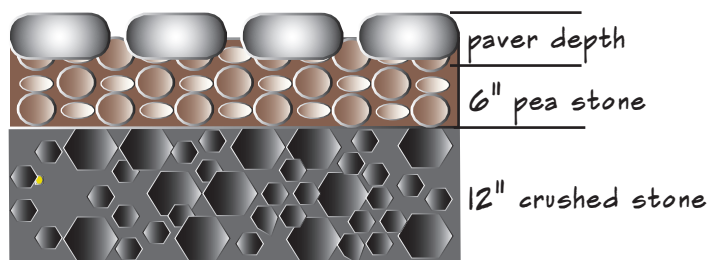
Figure 1. Pervious walkway profile.
