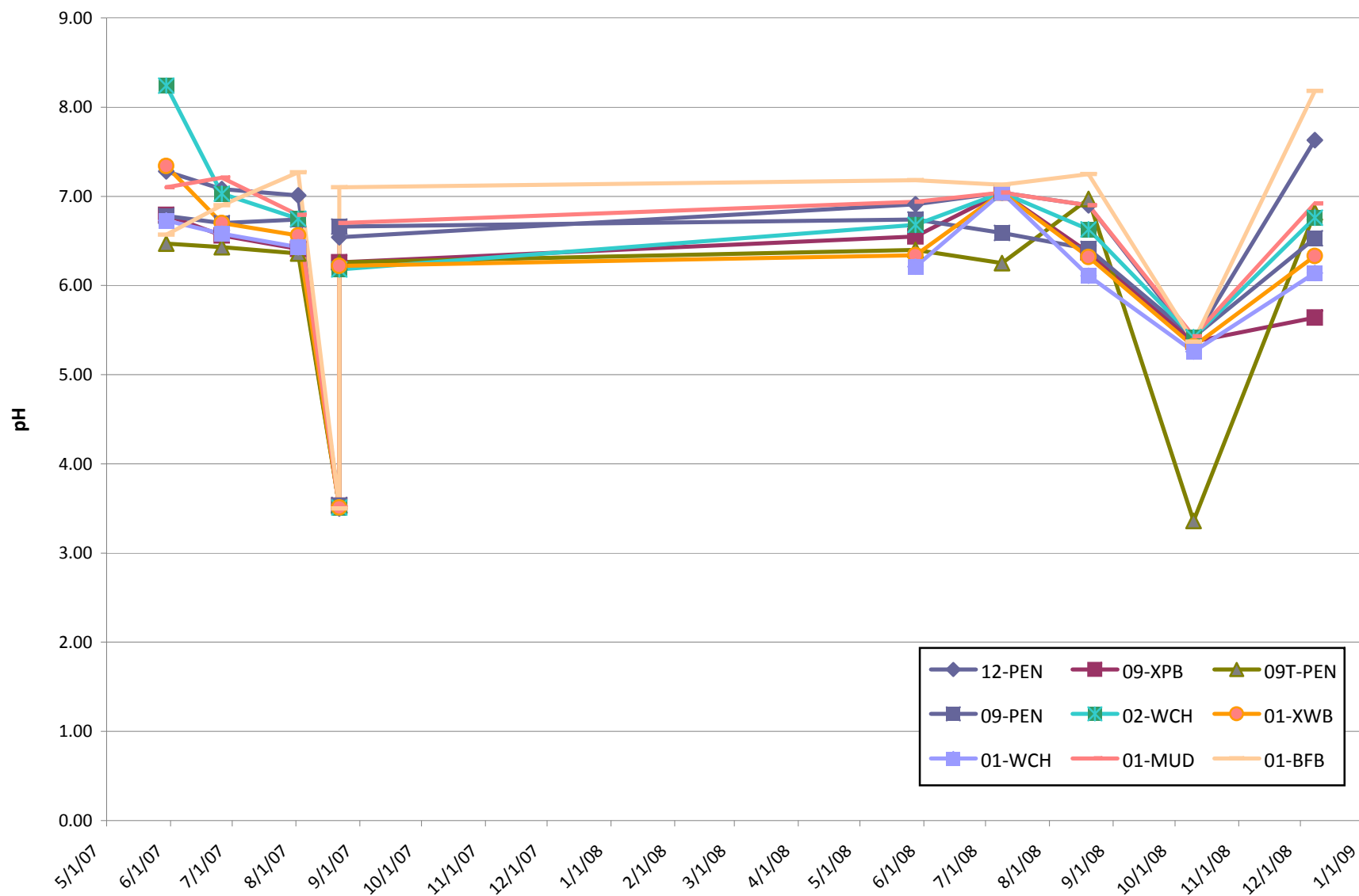
Dry Weather Sampling - pH 2007-2008
